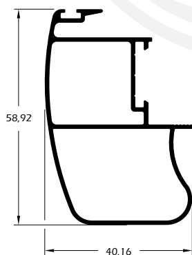
MG25-505 0,745 Kg/m Montante bi-tubular central externo
