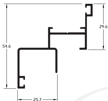
MG25-030 0,541 Kg/m Marco perimetral maxim-ar
